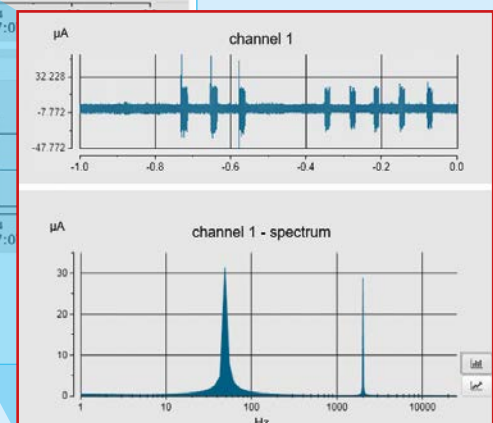
Fig. 23: Detail view of Channel 1 (amplitude, spectrum and frequency components)
