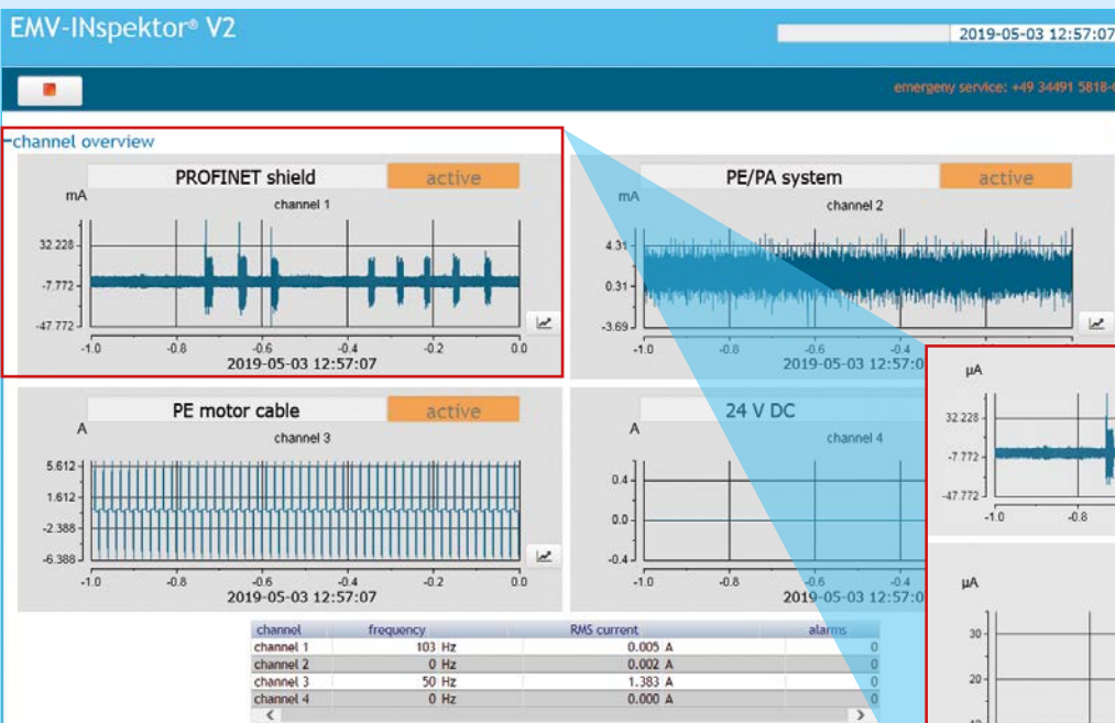
Fig. 24: Clear and detailed display of channels on the Web interface of EMV-INspektor® V2
