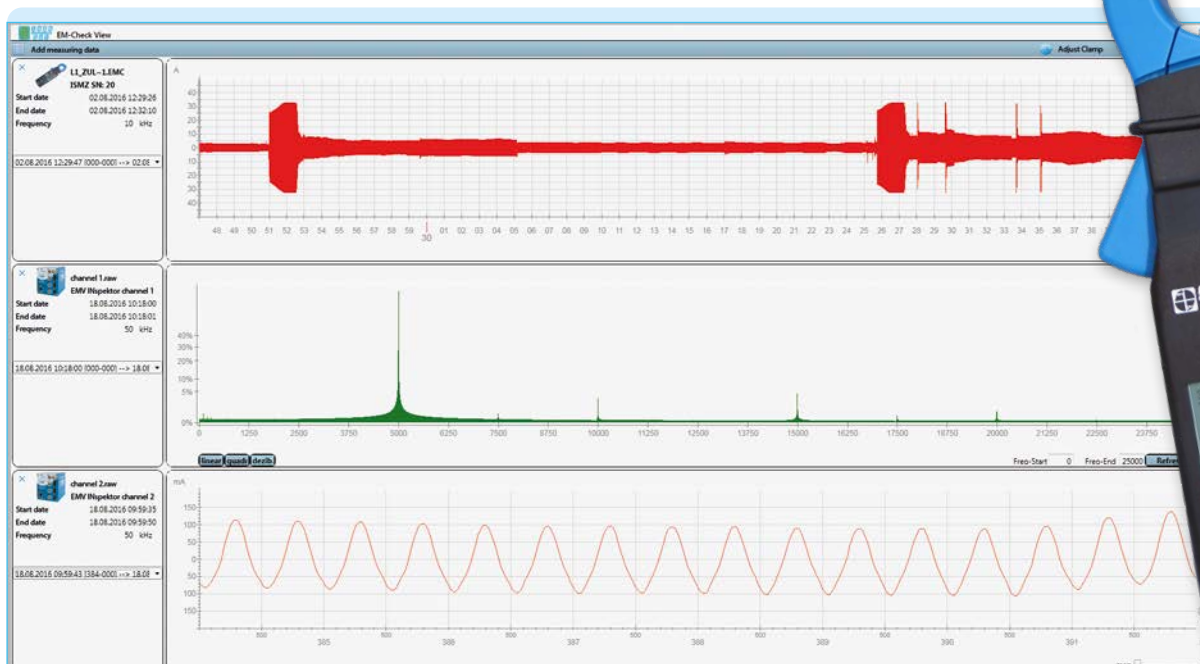
Fig. 20: Display of ISMZ measurement data by EmCheck® View
