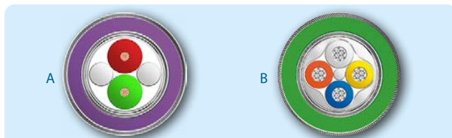
Fig. 13: Cross-sections PROFIBUS cable +FE (A), PROFINET cable +FE (B)
