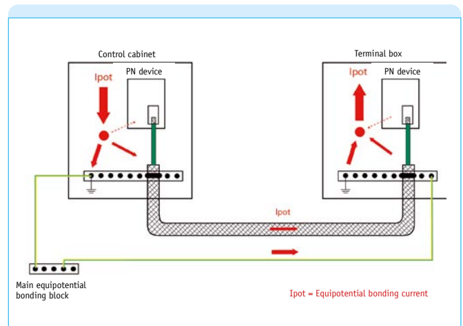
Fig. 15: Function 2 – Additional functional bonding
