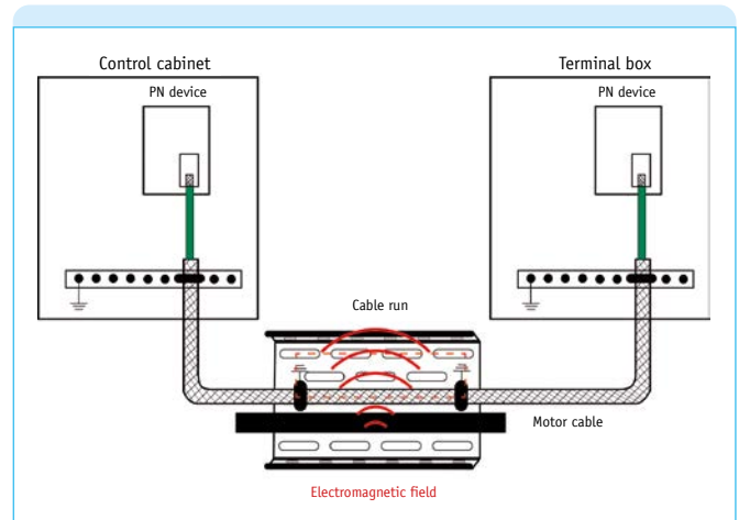
Fig. 14: Function 1 – Additional shield in environment with heavy field
