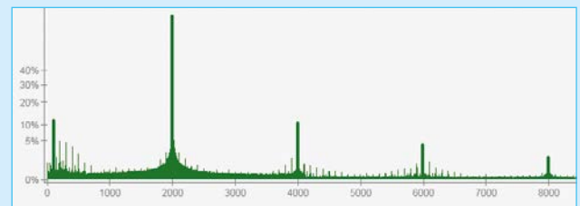
Fig. 22: Display of spectrum with 50 Hz and superimposed 2 kHz
