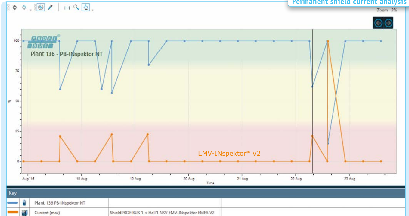
Fig. 25: Permanent shield current analysis compared to PROFIBUS condition graph
