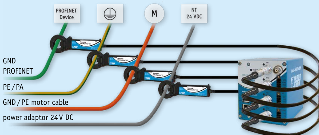
Fig. 21: Application example EMV-INSpektor® V2
